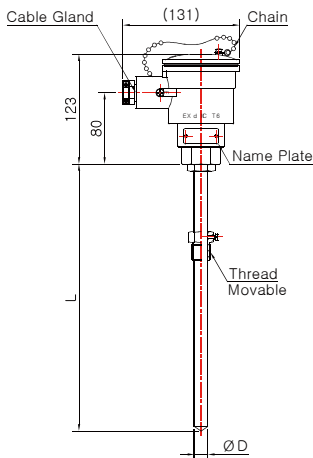
Model No. DS-3042E-3 (Sheath)
