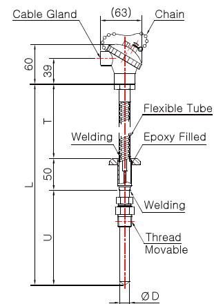
Model No. DS-3049S-3 (Sheath)
