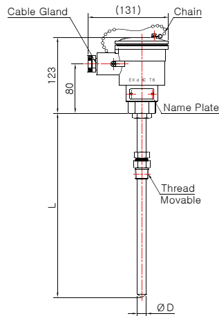
Model No. DS-3042E-4 (Sheath)
