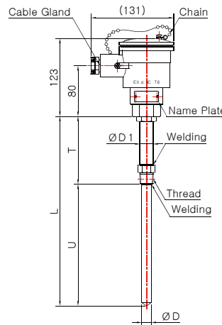
Model No. DS-3043E (Sheath)
