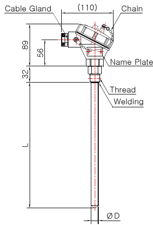
Model No. DS-3041W-2 (Sheath)
