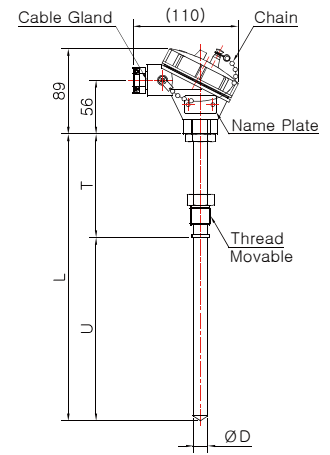
Model No. DS-3042W-2 (Sheath)
