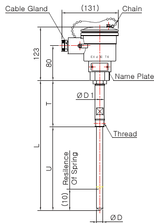
Model No. DS-3044E-1-1 (Sheath Spring Load)
