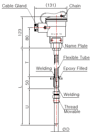
Model No. DS-3049SE-3 (Sheath)
