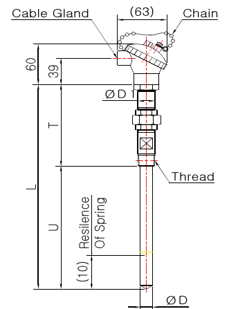
Model No. DS-3044S-2-1 (Sheath Spring Load)
