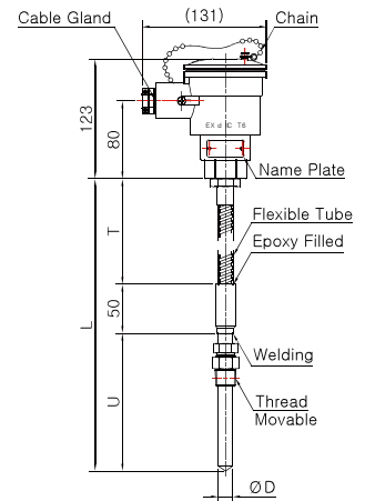
Model No. DS-3049E-1 (Sheath)
