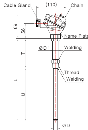
Model No. DS-3043W (Sheath)
