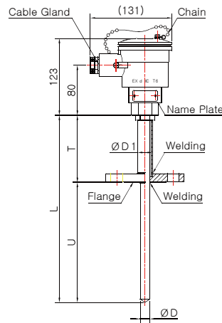
Model No. DS-3046E-1 (Sheath)
