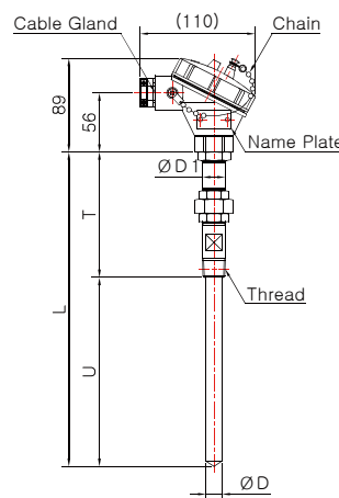
Model No. DS-3044W-2 (Sheath)
