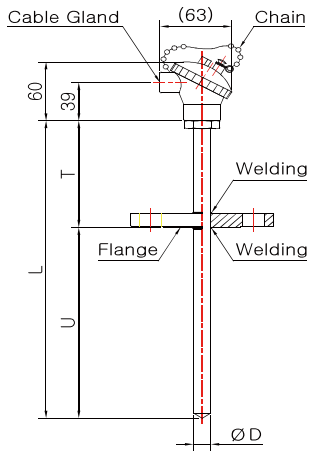
Model No. DS-3045S (Sheath)
