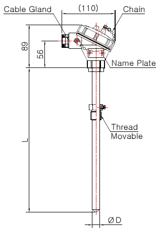
Model No. DS-3042W-3 (Sheath)
