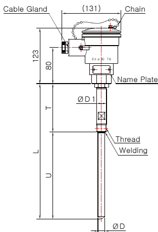
Model No. DS-3044E-1 (Sheath)
