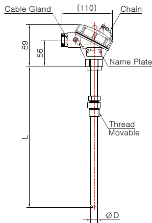
Model No. DS-3042W-4 (Sheath)
