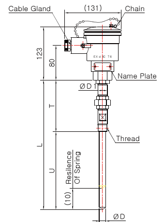
Model No. DS-3044E-2-1 (Sheath Spring Load)
