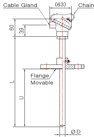
Model No. DS-3045S-1 (Sheath)
