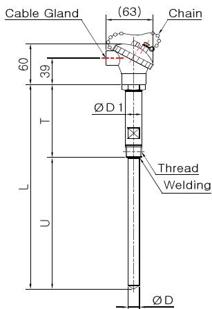
Model No. DS-3044S-1 (Sheath)
