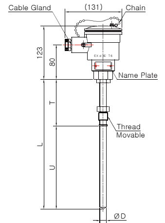
Model No. DS-3042E-2 (Sheath)
