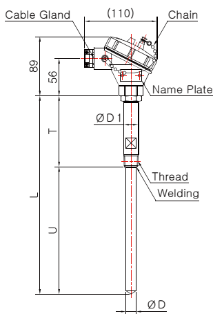
Model No. DS-3044W-1 (Sheath)
