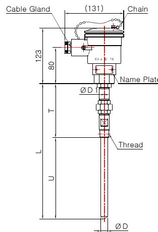
Model No. DS-3044E-2 (Sheath)
