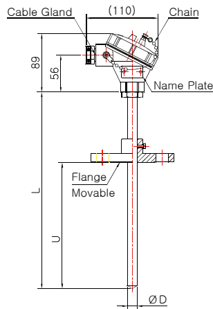
Model No. DS-3045W-1 (Sheath)
