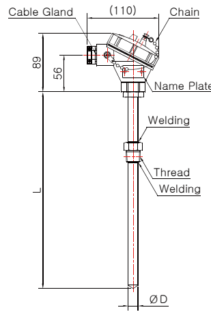
Model No. DS-3042W-1 (Sheath)
