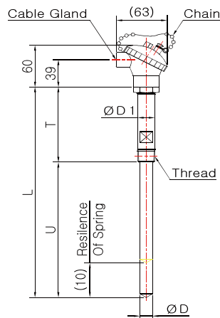
Model No. DS-3044S-1-1 (Sheath Spring Load)
