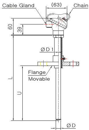
Model No. DS-3046S-2 (Sheath)
