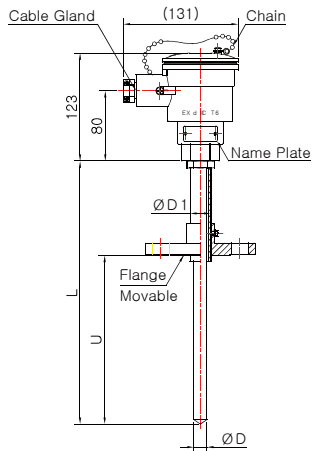
Model No. DS-3046E-2 (Sheath)
