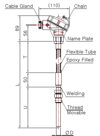
Model No. DS-3049W-1 (Sheath)
