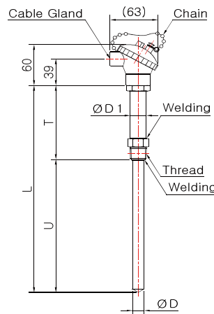
Model No. DS-3043S (Sheath)
