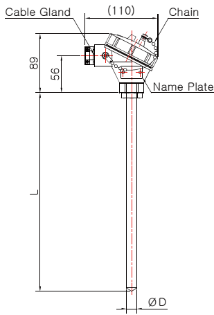
Model No. DS-3041W (Sheath)
