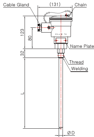
Model No. DS-3041E-2 (Sheath)
