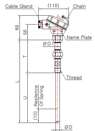
Model No. DS-3044W-2-1 (Sheath Spring Load)
