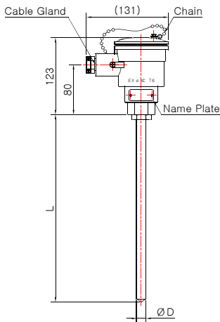
Model No. DS-3041E (Sheath)
