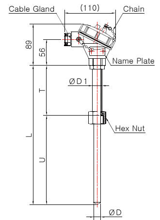
Model No. DS-3043W-1 (Sheath)
