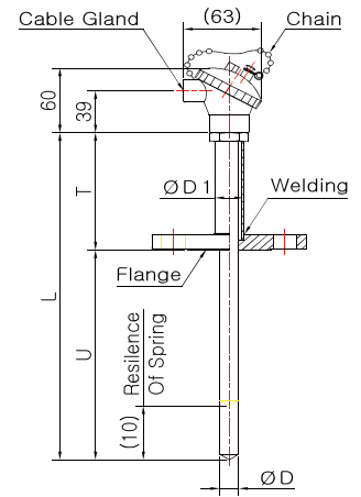
Model No. DS-3046S-1-1 (Sheath Spring Load)
