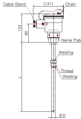
Model No. DS-3042E-1 (Sheath)
