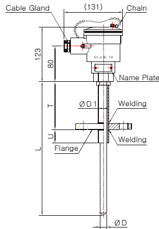
Model No. DS-3046E-3 (Sheath)
