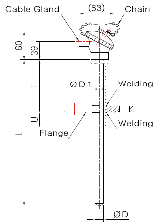
Model No. DS-3046S-3 (Sheath)
