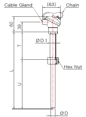
Model No. DS-3043S-1 (Sheath)
