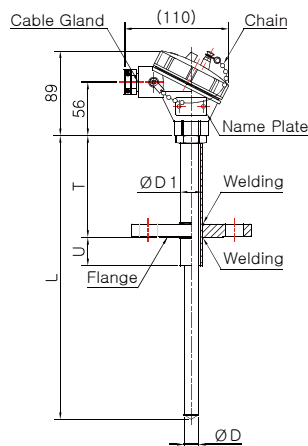
Model No. DS-3046W-3 (Sheath)
