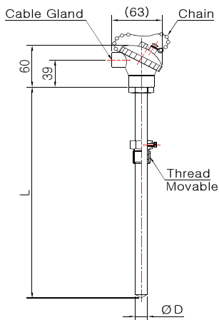
Model No. DS-3042S-3 (Sheath)
