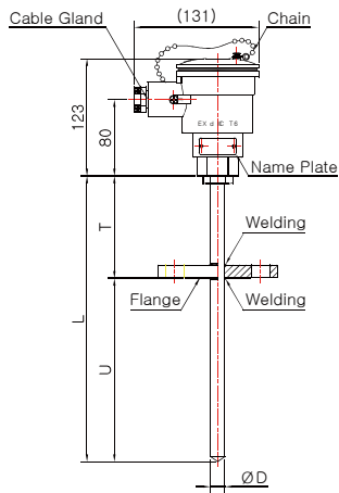
Model No. DS-3045E (Sheath)
