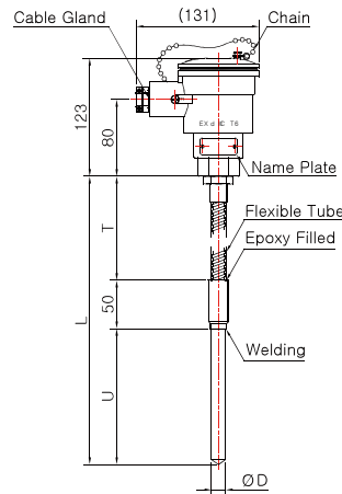
Model No. DS-3049E (Sheath)
