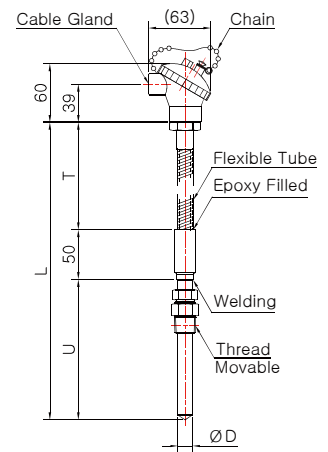
Model No. DS-3049S-1 (Sheath)
