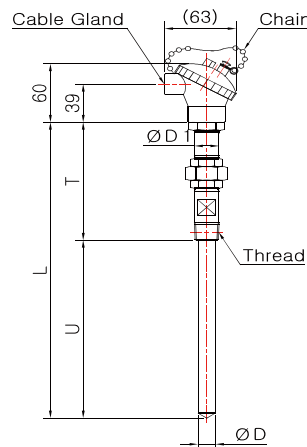
Model No. DS-3044S-2 (Sheath)
