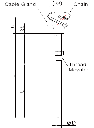
Model No. DS-3042S-2 (Sheath)
