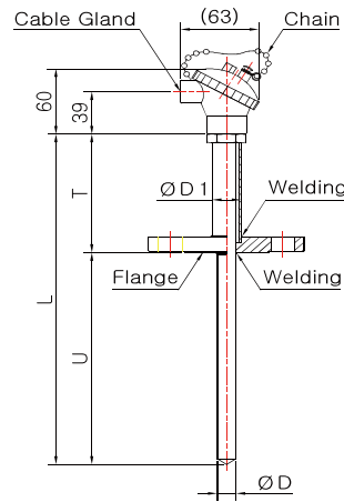
Model No. DS-3046S-1 (Sheath)
