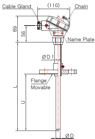
Model No. DS-3046W-2 (Sheath)
