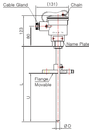
Model No. DS-3045E-1 (Sheath)
