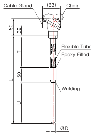
Model No. DS-3049S (Sheath)
