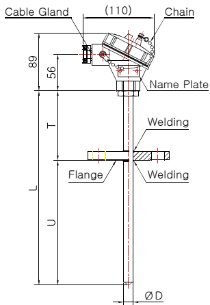
Model No. DS-3045W (Sheath)
