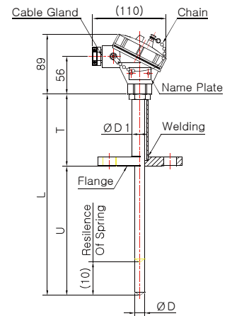
Model No. DS-3046W-1-1 (Sheath Spring Load)
