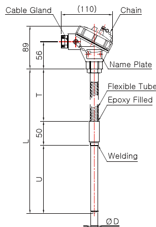
Model No. DS-3049W (Sheath)
