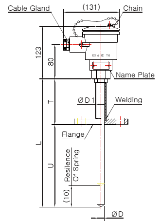
Model No. DS-3046E-1-1 (Sheath Spring Load)
