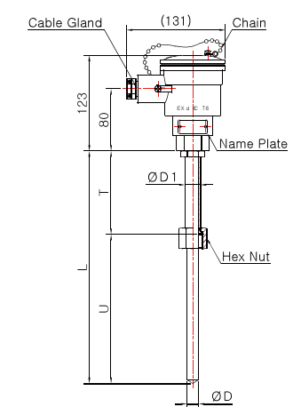
Model No. DS-3043E-1 (Sheath)
