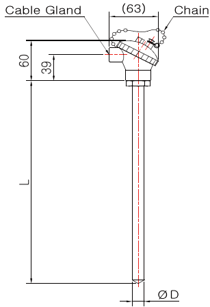
Model No. DS-3041S (Sheath)
