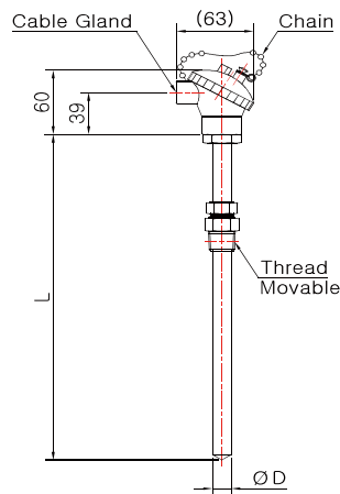
Model No. DS-3042S-4 (Sheath)
