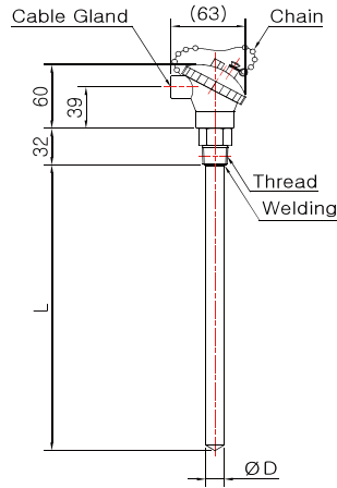
Model No. DS-3041S-2 (Sheath)
