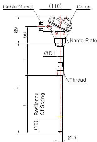
Model No. DS-3044W-1-1 (Sheath Spring Load)
