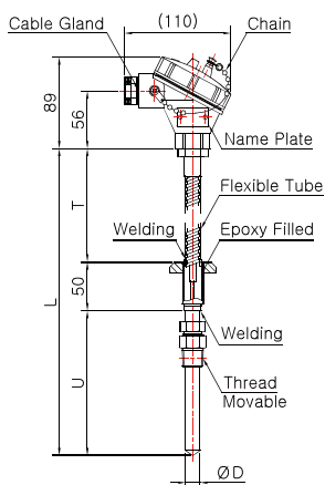
Model No. DS-3049SW-3 (Sheath)
